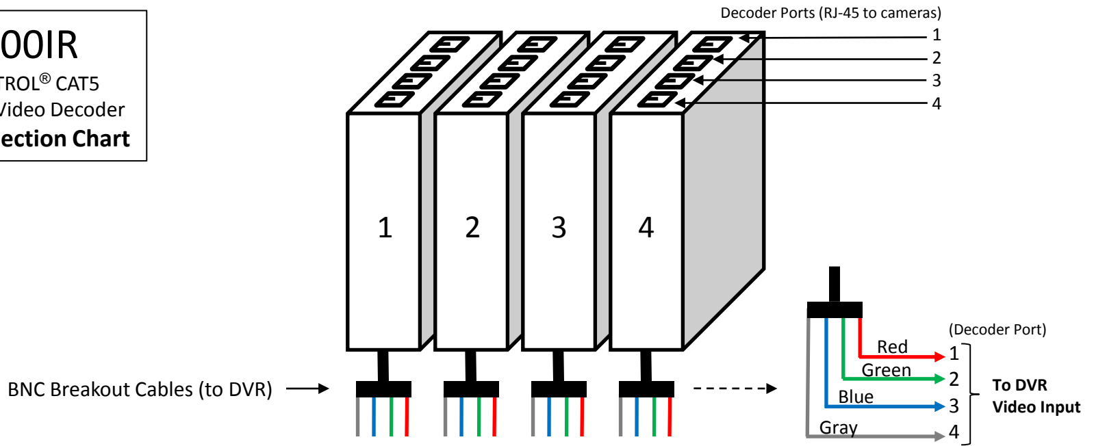
Decoder Port - to - DVR/Camera Connection Chart
